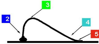
Fig. 9: Criteria to establish failure mode for wire bond pull testing
