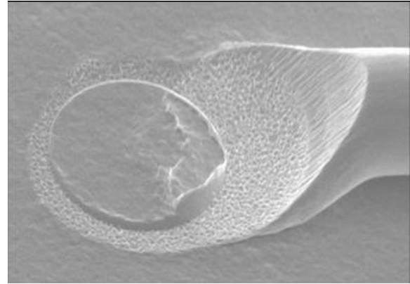
Fig. 12: Typical copper wire wedge bond
