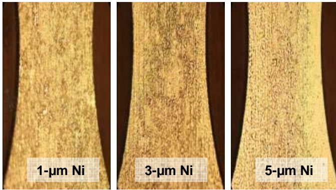
Fig 14. High-phosphorus ENIG deposit after 2-mm wire pull/bend test showing defect-free surface
