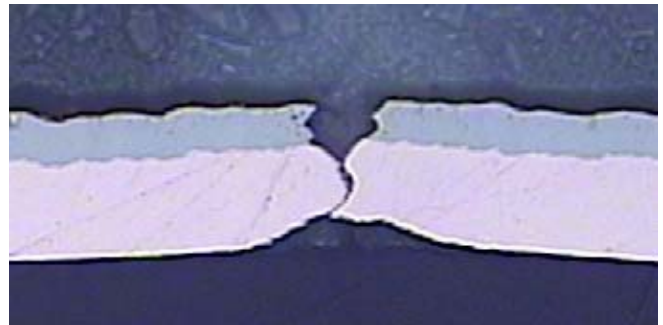
Fig 13. Cross section of 5- \mu\text{m} medium-phosphorus ENIG deposit on copper following 2-mm wire pull/bend test
