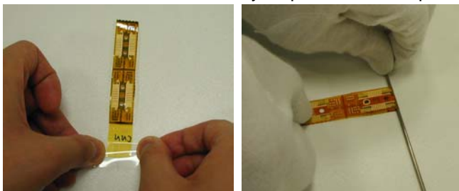
Fig 11. Securing the flex circuit sample (left) and performing the 2-mm wire pull/bend test (right)
