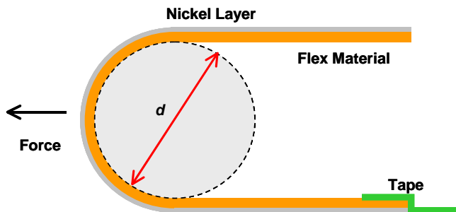
Fig 10. Wire pull/bend test for flexible circuits
