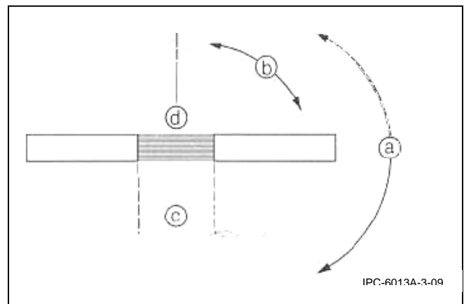
Fig 7. Bending test according to IPC-6013A
