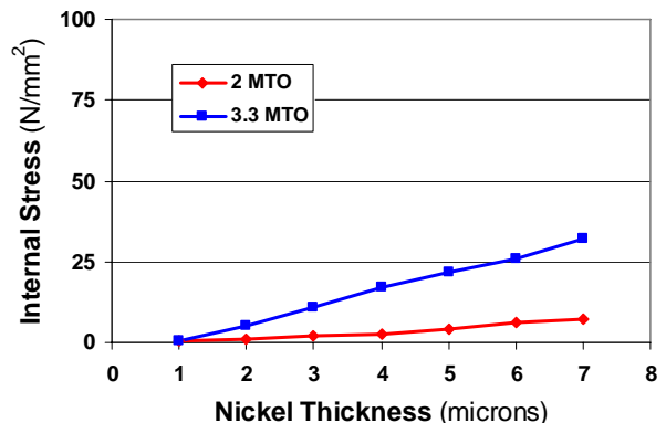
Fig18. Relationship of internal stress and nickel thickness for high-P nickel deposit
