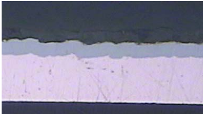
Fig 15. Cross section of 5-µm high-phosphorus ENIG deposit on copper following 2-mm wire pull/bend test
