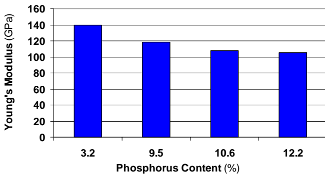
Fig 19. Comparison of Young's Modulus vs. phosphorus content of different electroless nickel deposits
