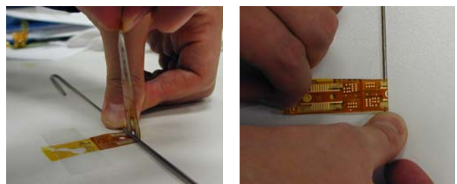
Fig 8. Performing the 90 °C bend test (left) and 180° bend test (right)
