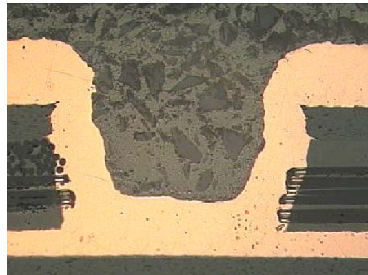
Figure 7 – Flex-rigid permanganate desmeared Figure 8 – Blind microvia flex permanganate desmeared
