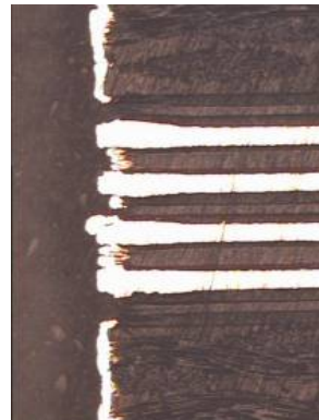
Figure 6 – Permanganate Desmear + Electroless
