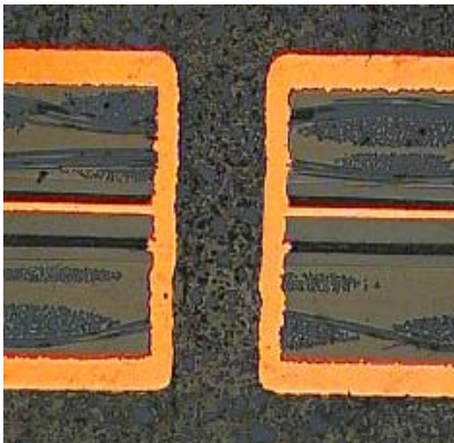
Figure 7 – Flex-rigid permanganate desmeared Figure 8 – Blind microvia flex permanganate desmeared
