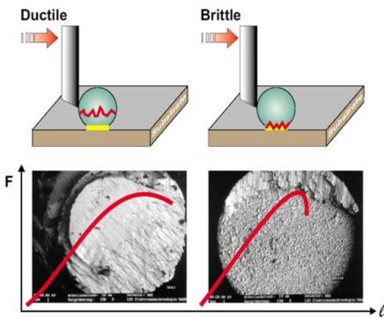
Fig. 3 Schematic diagrams of ball shear test and SEM micrographs of ductile and brittle fracture.
