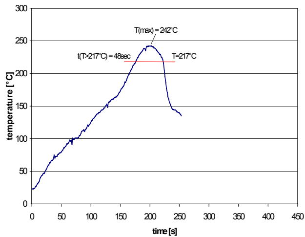
Fig. 16 Reflow profile for Sn-Ag-Cu (lead-free) solder paste
