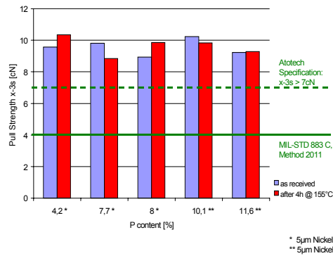
Fig. 28 Comparison of different bulk nickel phosphorus contents to aluminum-wire pull strength.
