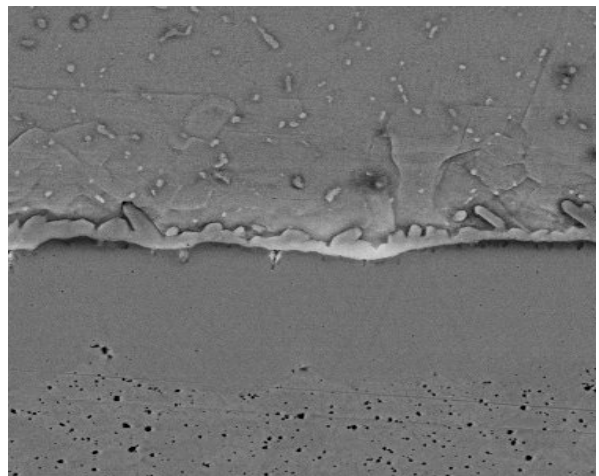
Fig.19: SEM image of IMC cross-section after thermo cycling (8.0wt % P Nickel layer)
