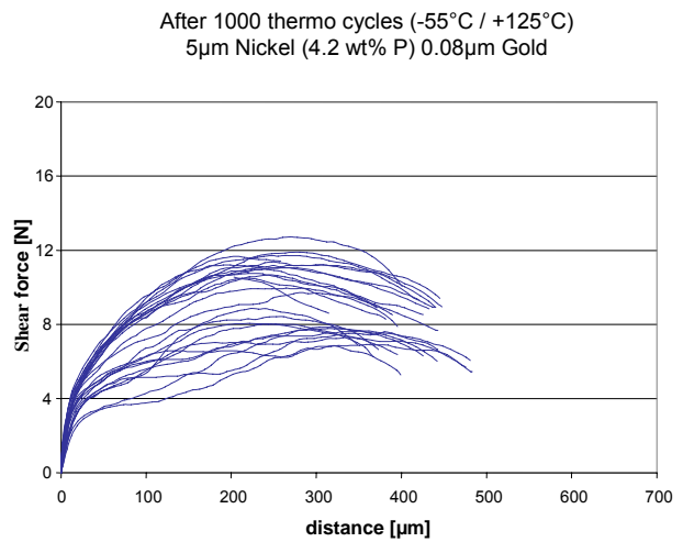
Fig. 11 Ball shear tests on 600- \mu m pads (after thermo-cycling) 5 \mu m NiP (4.2% P-content), 0.08 \mu m gold
