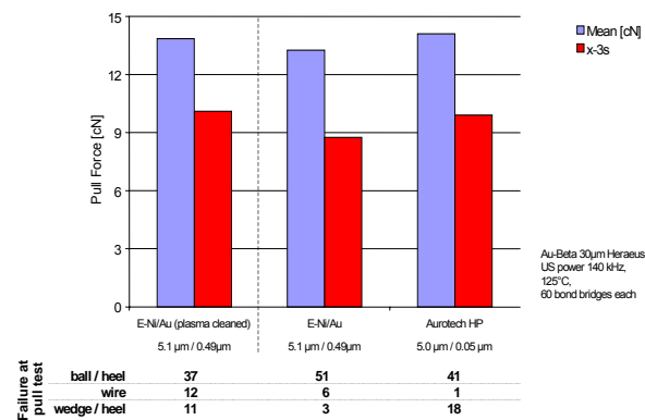
Fig. 29 Comparison of two different nickel/gold systems to gold-wire pull strength
