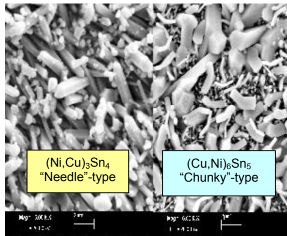
Fig. 23 Different types of IMC produced after 400 thermo-cycles
